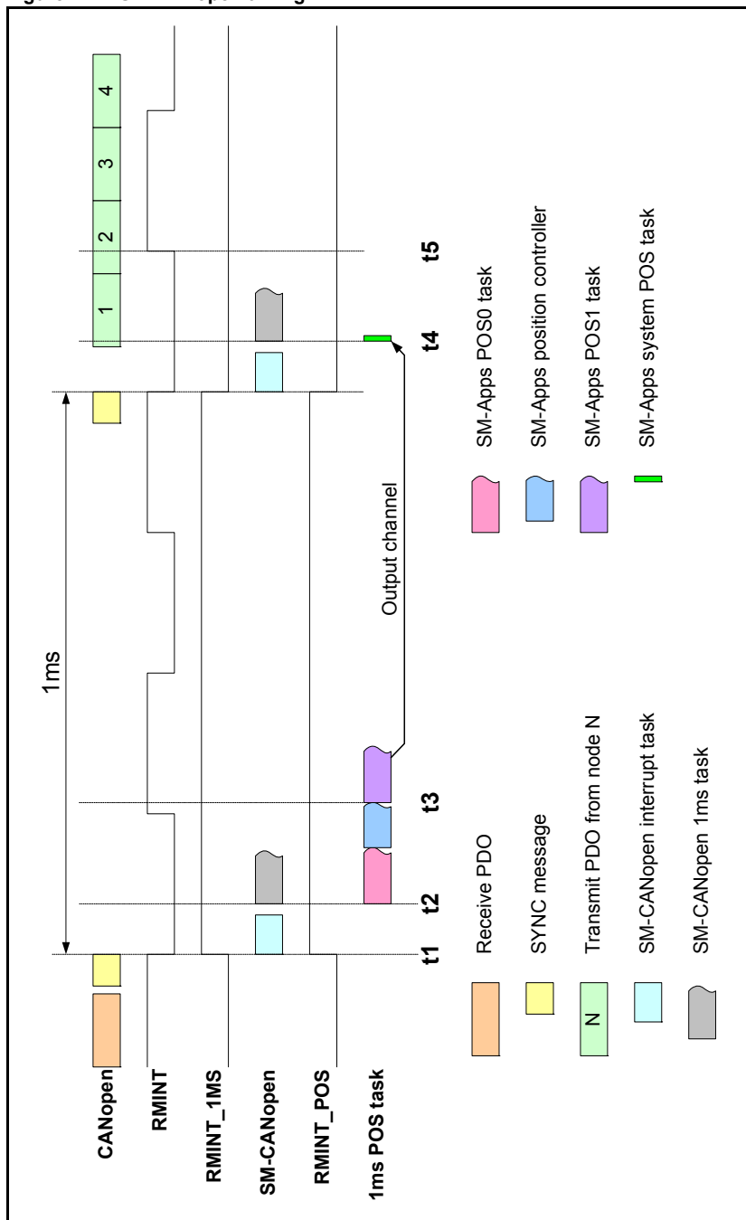
Figure 11-4 SM-CANopen timing
